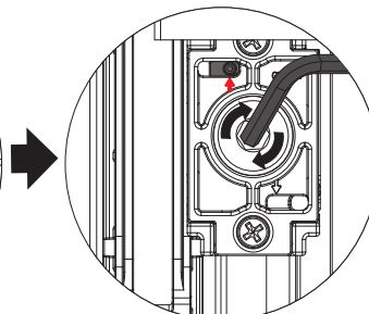
Turn the screw clockwise with a 3mm allen key to engage the locking devices on the top rollers of the outer and inner doors
