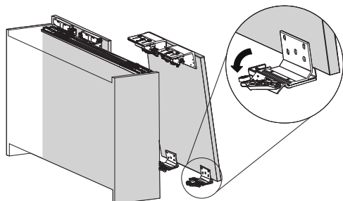
Disengage the locking device on bottom roller before mounting the outer door
